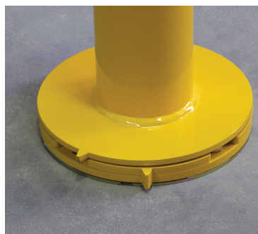
Bollard installed into shoe.
