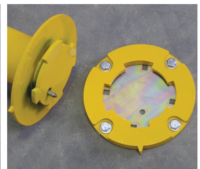
Bollard to shoe interlock (SMCLH).
